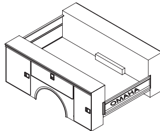
12 GA. TREADPLATE STEEL OVERLAY ON REAR END PANELS FURNISHED STANDARD WITH 6,000# CRANE REINFORCING STREETSIDE CURBSIDE
