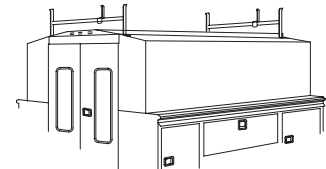
LR-7 HI ROOF/OSV OVERHEAD LADDER RACK
