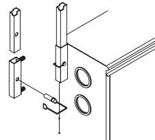
LR-4 QUICK REMOVAL BRACKETS
