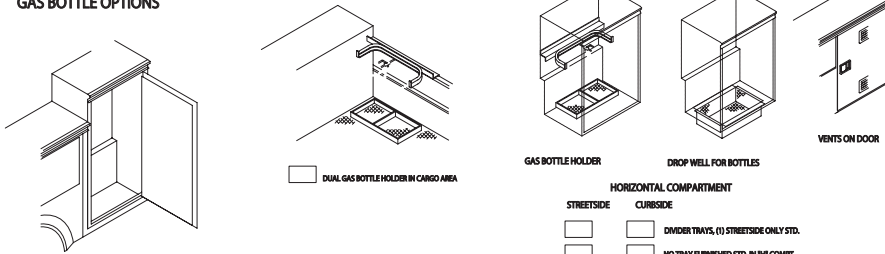
FRONT RAISED COMPARTMENT 50" HIGH 60" HIGH 66" HIGH
